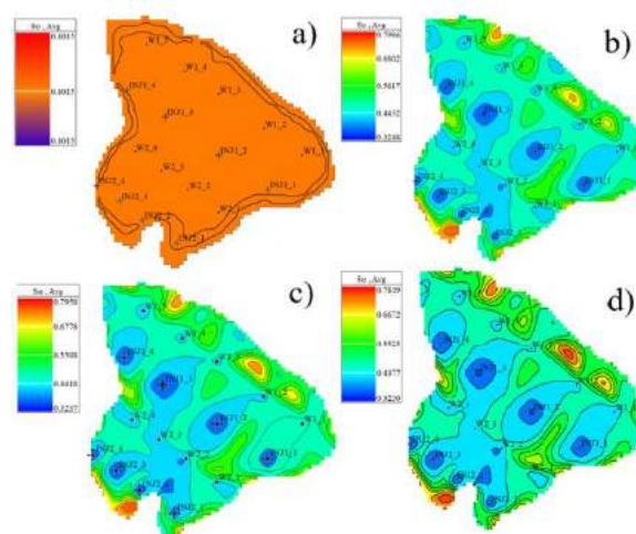
Fig. 3. Map of the initial oil saturation of the development object; b), c), d) residual oil saturation during the transition to the injection of LMW for the value of water cut 60%, 80%, 90%, respectively
