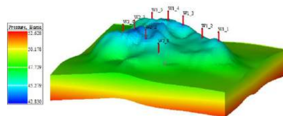
Fig. 1. Geological and hydrodynamic model: 3D-map of the distribution of the initial reservoir pressure by blocks
