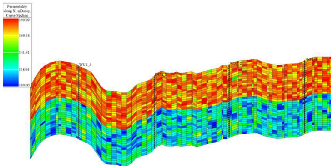
Fig. 5. Section of the Model before using low- mineralized waterflooding: permeability distribution map
