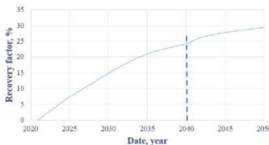
Fig. 7. Change in ORF, % (up to 2040 flooding with high-salinity water, after injection of LMW)
