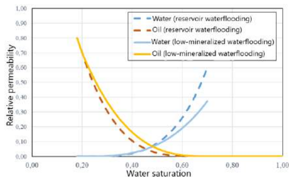
Fig. 2. RP curves used in the model
