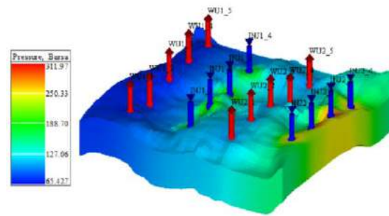
Fig. 4. Geological and hydrodynamic model: 3D-map of the distribution of the initial reservoir pressure by blocks
